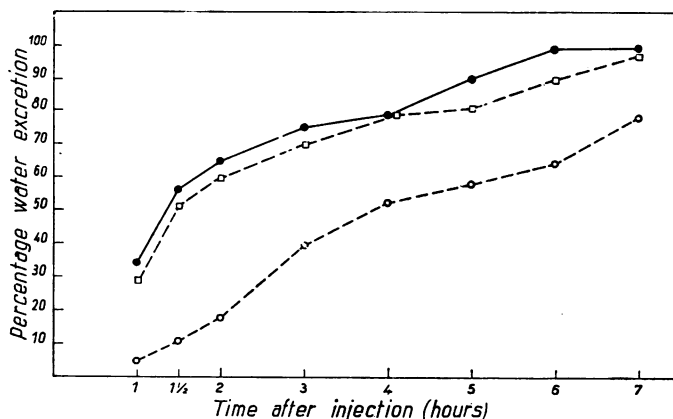
FIG. 2.—The antidiuretic effect of rabbit serum extract, 1.0 ml. per 100 g., before (○---○) and after (□---□) treating with diazotized p -nitroaniline. ●---● 1 ml. saline per 100 g. Each point of the curves is the mean of results from 2 groups of 4 animals each.
